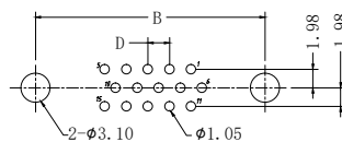
P.C B LAYOUT (15PIN) GENERAL TOLERANCE: ±0.05
