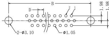
P.C B LAYOUT (26~62PIN) GENERAL TOLERANCE: ±0.05
