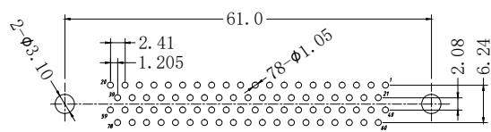
P.C BOARD LAYOUT (78PIN) GENERAL TOLERANCE: ±0.05
