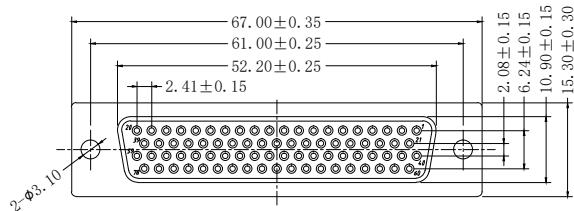
P.C B LAYOUT (26~62PIN) GENERAL TOLERANCE: ±0.05
